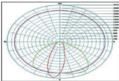
Luminous Flux OO Optic 3593lm
