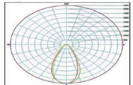
Luminous Flux WW Optic 3902lm
