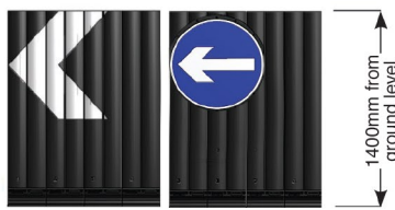
800mm Chevron without border
