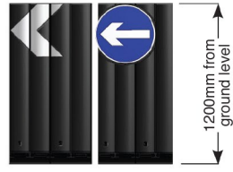
600mm Chevron without border
