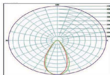
Luminous Flux WW Optic 3902lm
