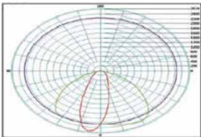
Luminous Flux OO Optic 3593lm
